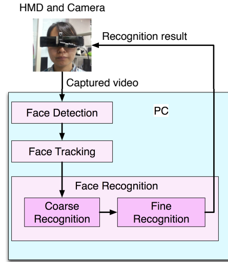
Figure 2: Procedure of the proposed face recognition system
