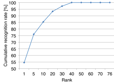
Figure 4: Cumulative recognition rates for the coarse face recognition
